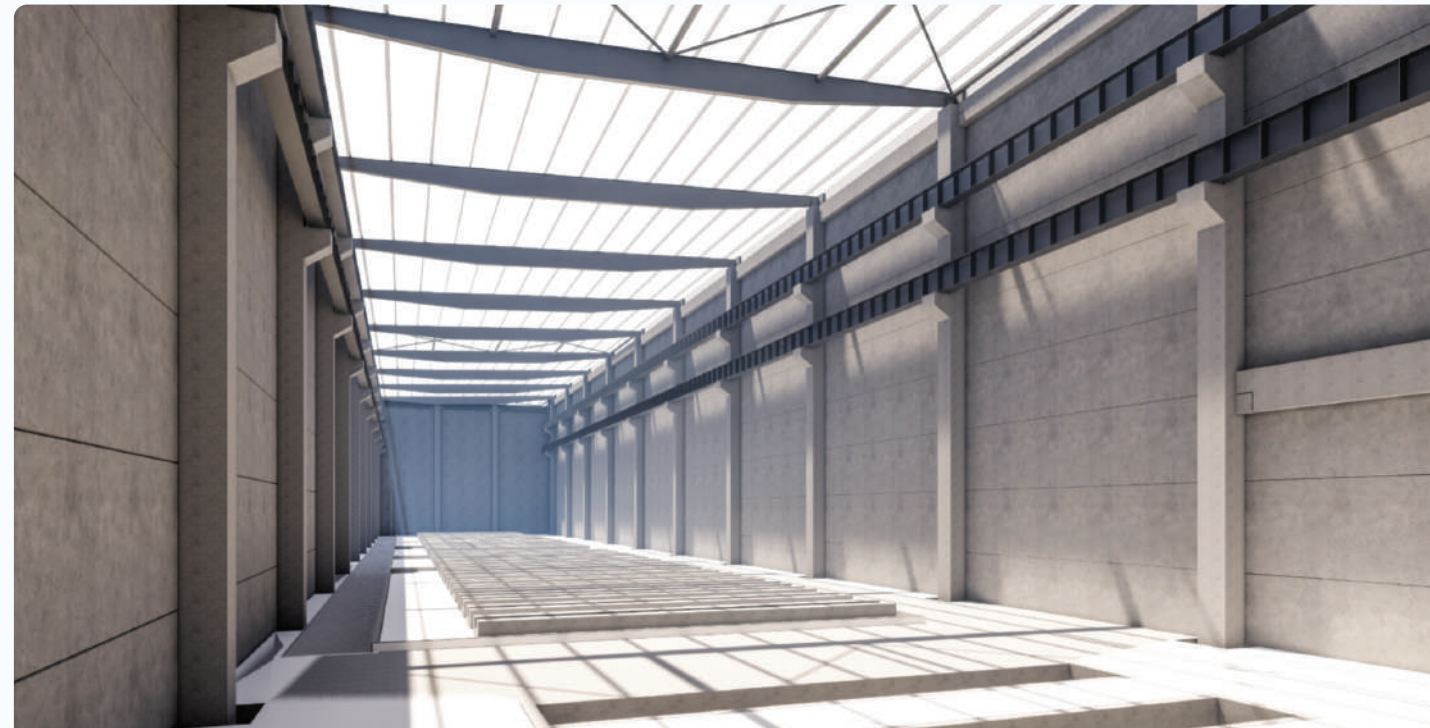
3D Model: Design of Precast Concrete Columns, Wall Panels
